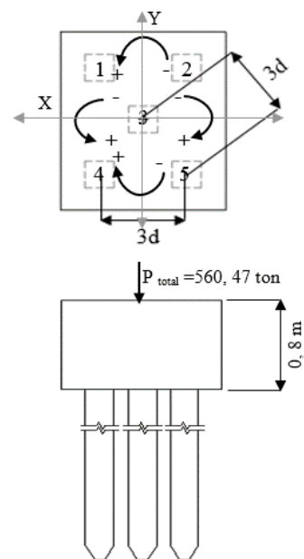
Gambar 4. Distribusi beban
