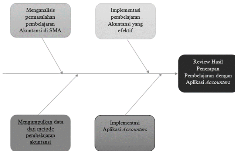
Gambar 1. Conceptual framework.
