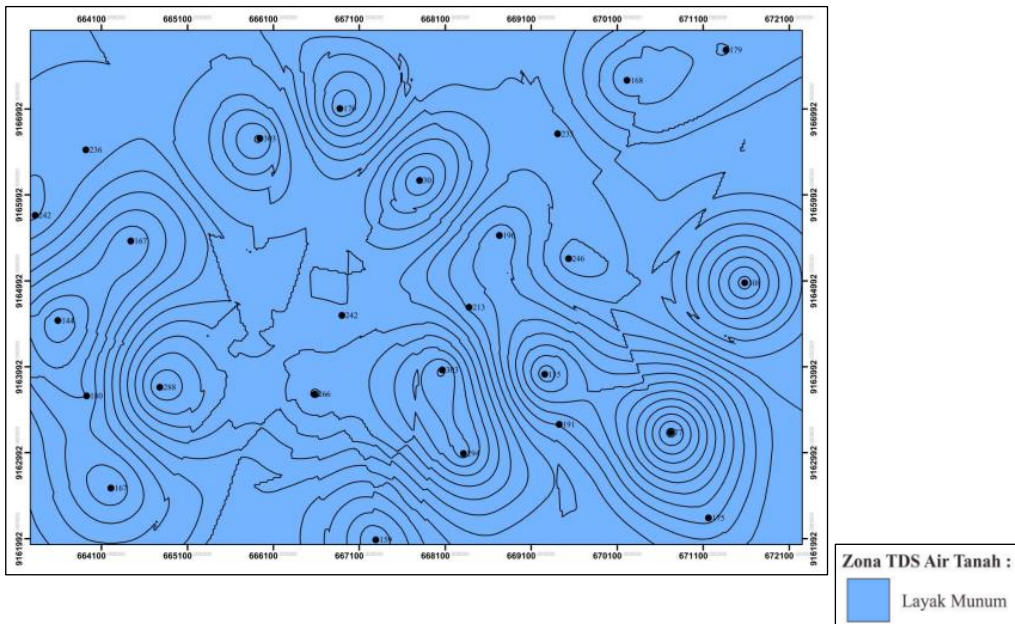
Gambar 5. Peta nilai Total Dissolved Solid (TDS) di lokasi penelitian
