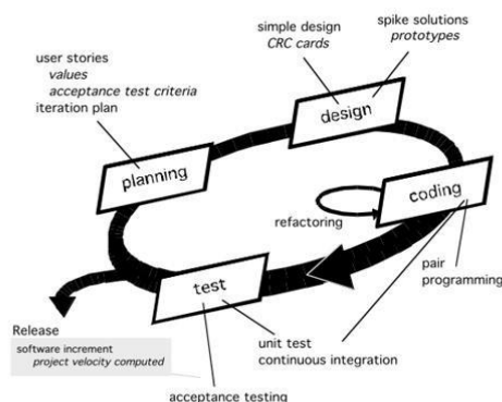
Gambar 1. Extreme programming
