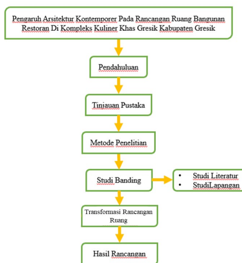
Gambar 1. Diagram Metode
