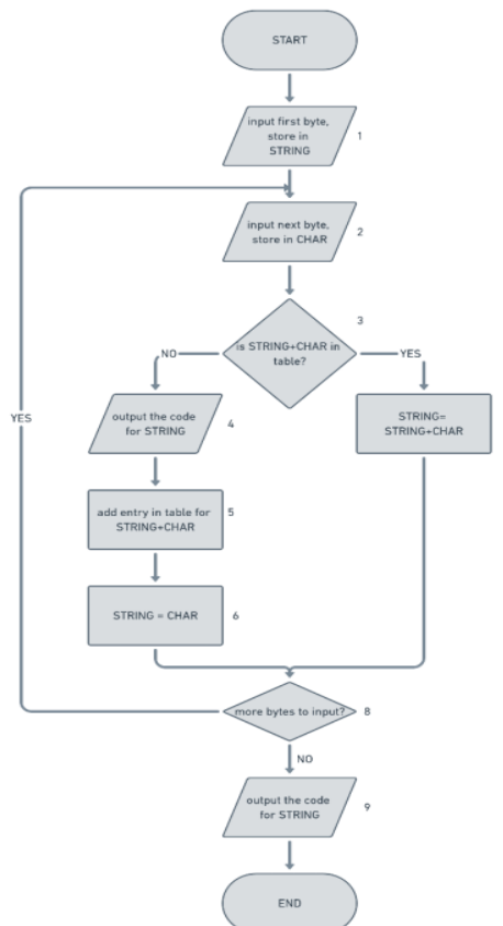
Gambar 3. Flowchart Algoritma LZW
