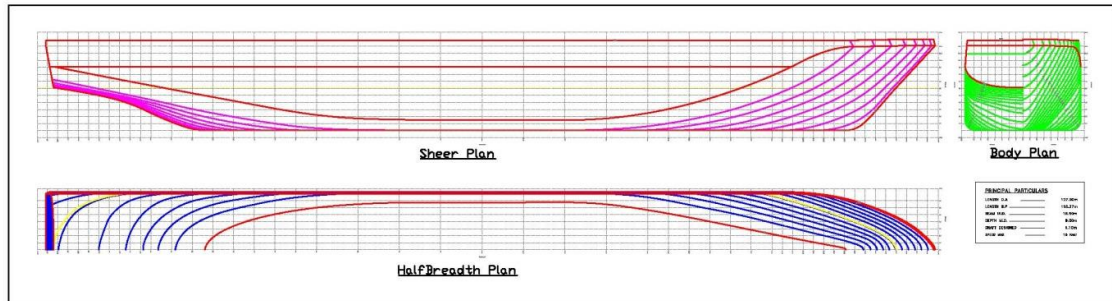
Gambar 1. Lines Plan Awal 127m
