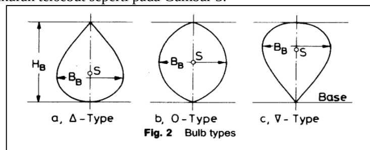
Gambar 3. bulb types
