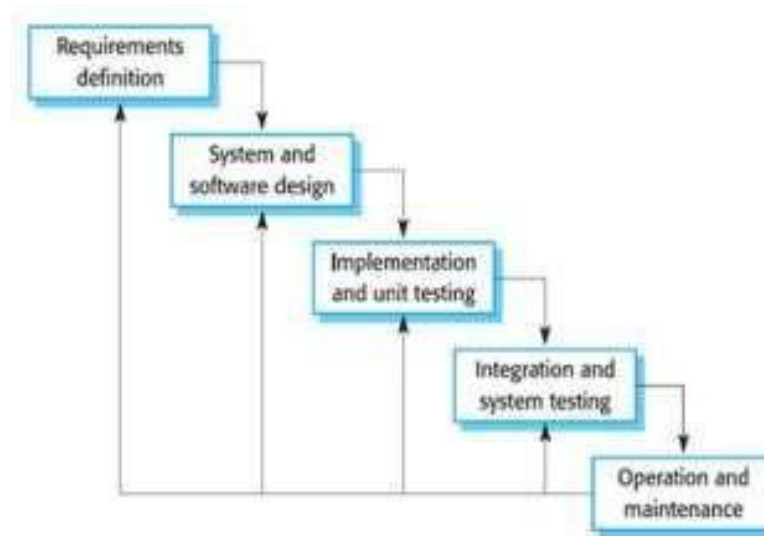
Gambar 1. Waterfall
