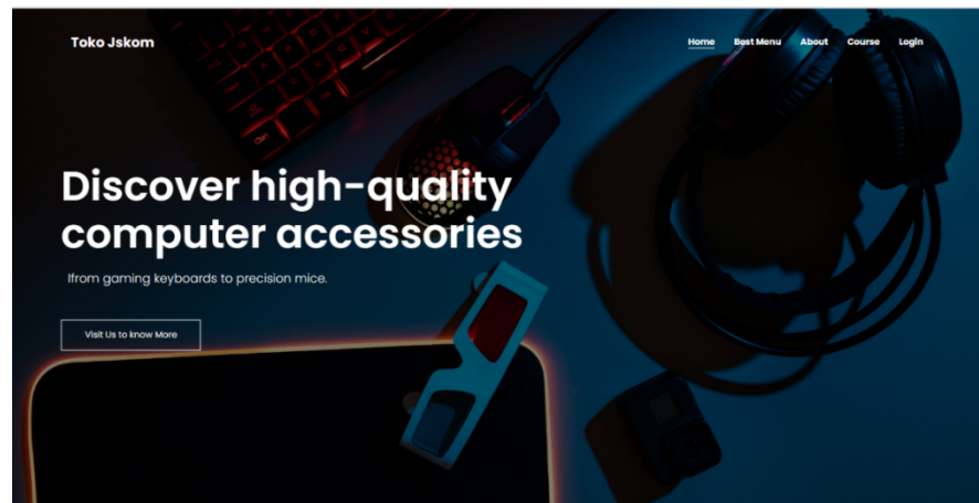
Gambar 4. Menu Dashboard
