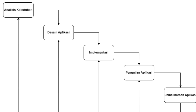
Gambar 1. model Waterfall .
