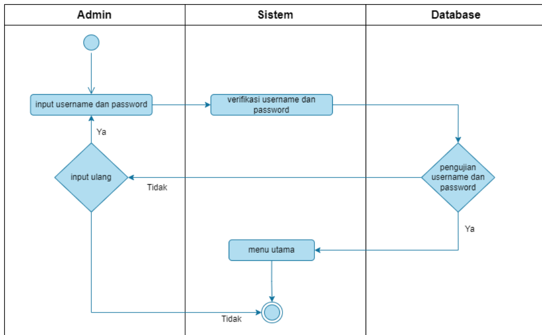
Gambar 5. Activity Login
