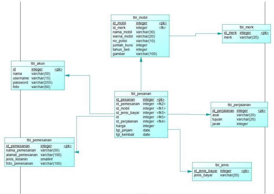
Gambar 3. Desain Database Pdm.
