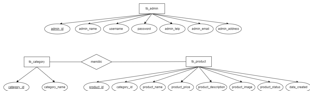
Gambar 4.1. class diagram
