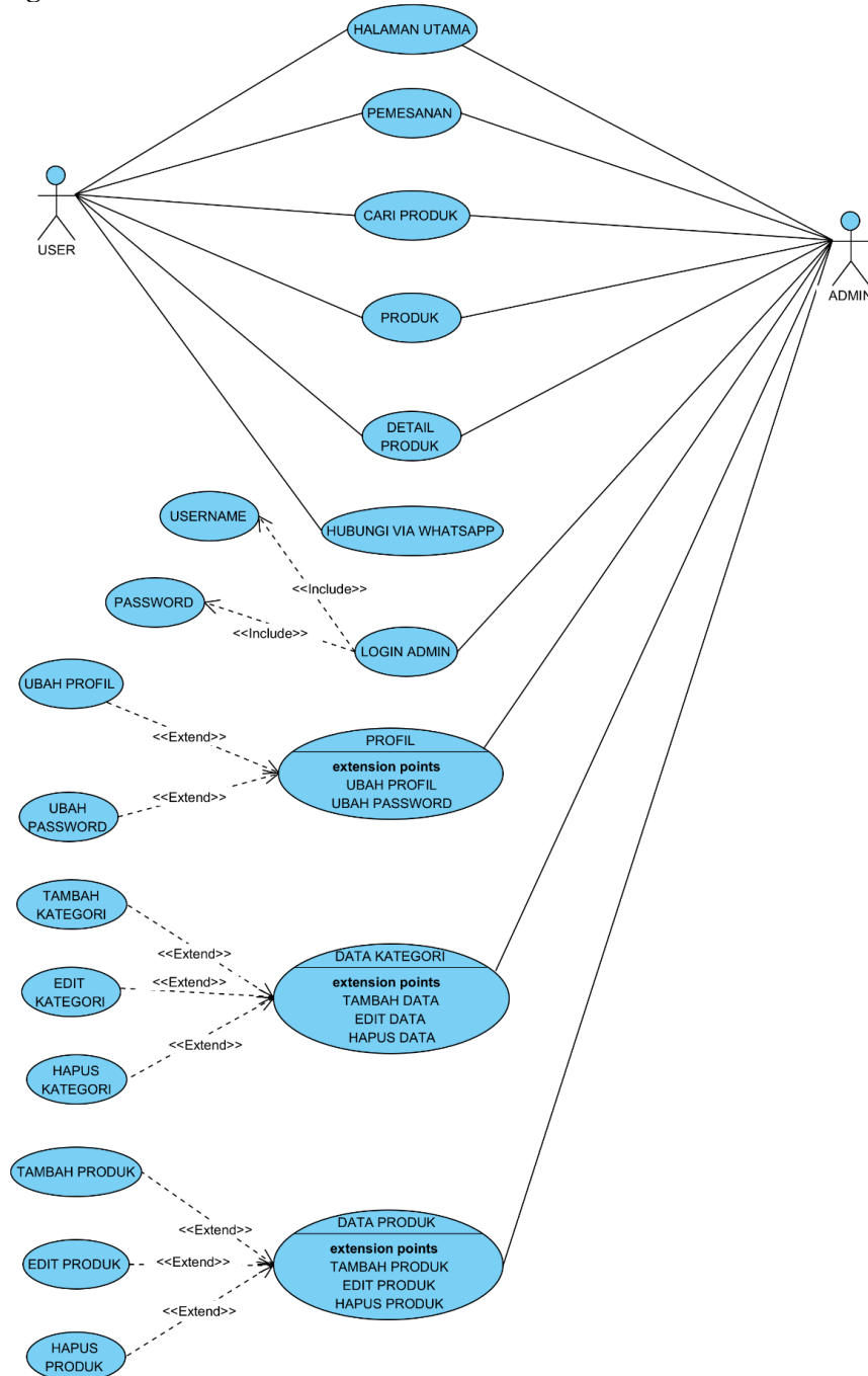
Gambar 1. Usecase Diagram
