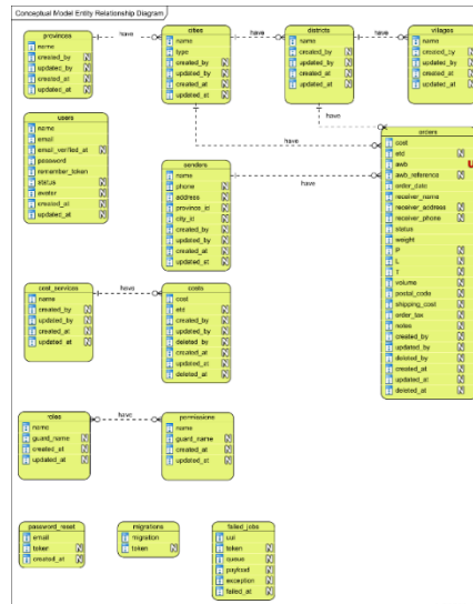
Gambar 2. Conceptual Data Model
