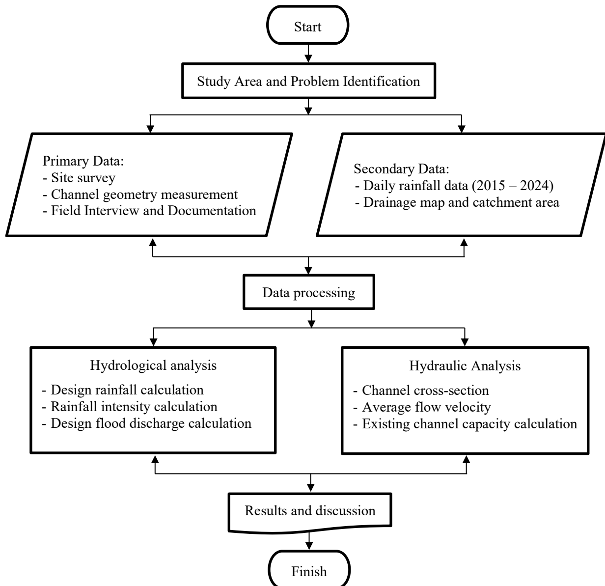
Figure 3. Research flowchart
