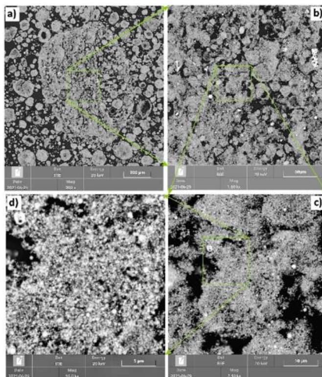
Figure 1 (a) Silica Smoking Micropellet, (b) Micropellet form at 1500x magnification, (c) Micropellet shape at 7500x, (d) magnification. Micropellet shape at 15000x magnification [3]
