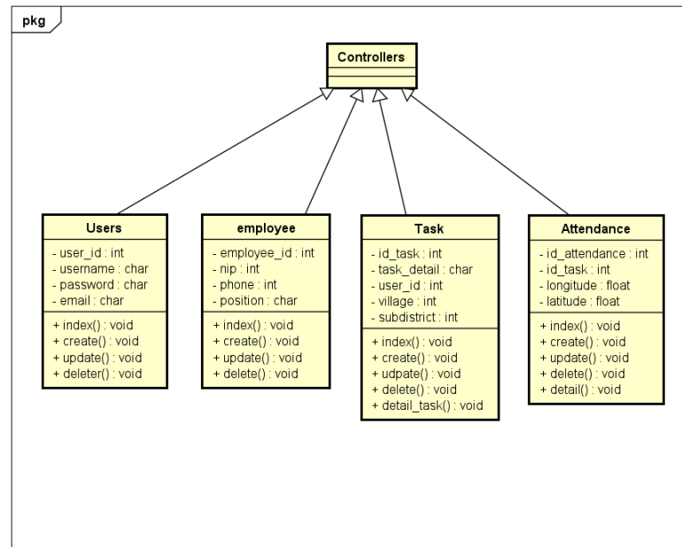
Fig 5. Class Diagram for web application
