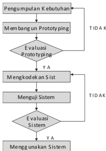
Gambar 1. Metode Prototyping
