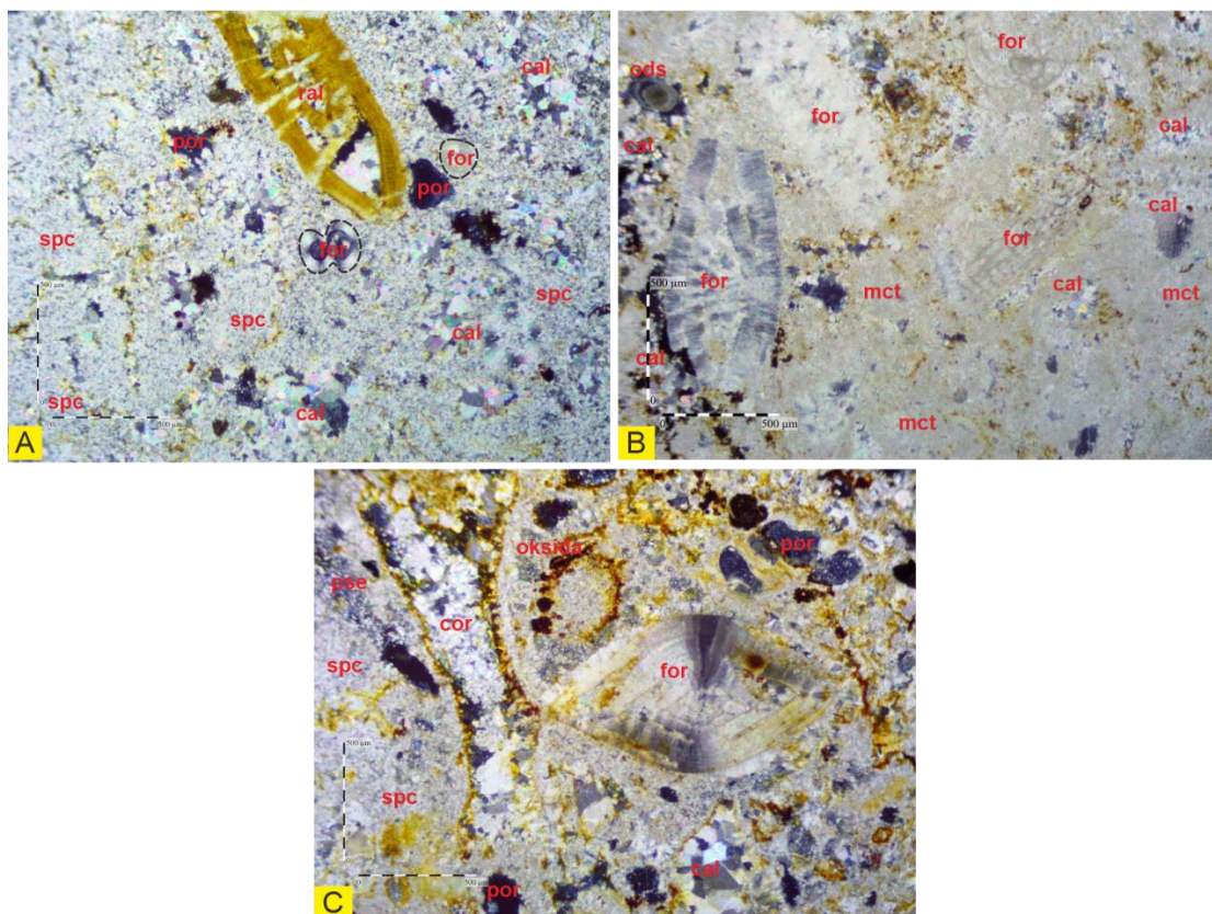
Gambar 6. Foto mikroskop batugamping daerah penelitian (A) Fasies Wackestone or floatstone which whole fossils , (B) Fasies Bioclastic packstone or wackestone with worn skeletal grain , (C) Fasies Grainstone or packstone with abundant foram
