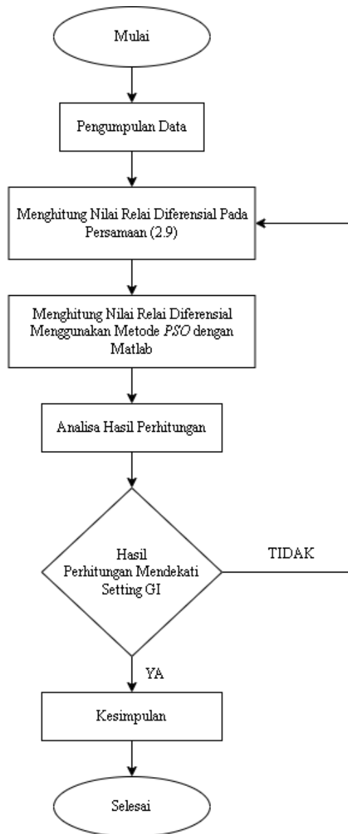
Gambar 1 Flowchart Penelitian
