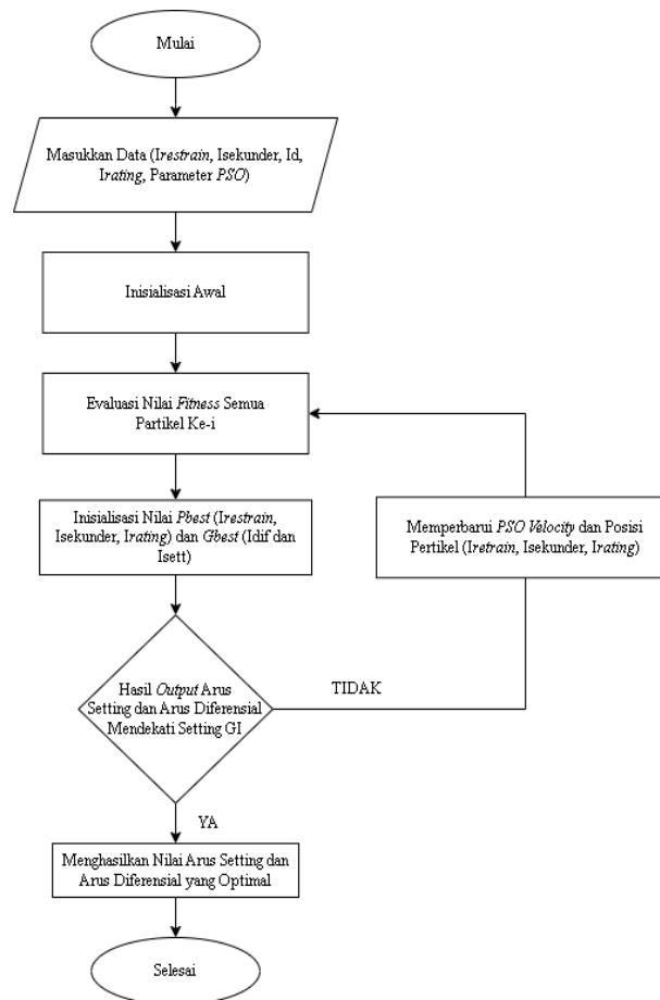
Gambar 2 Flowchart PSO
