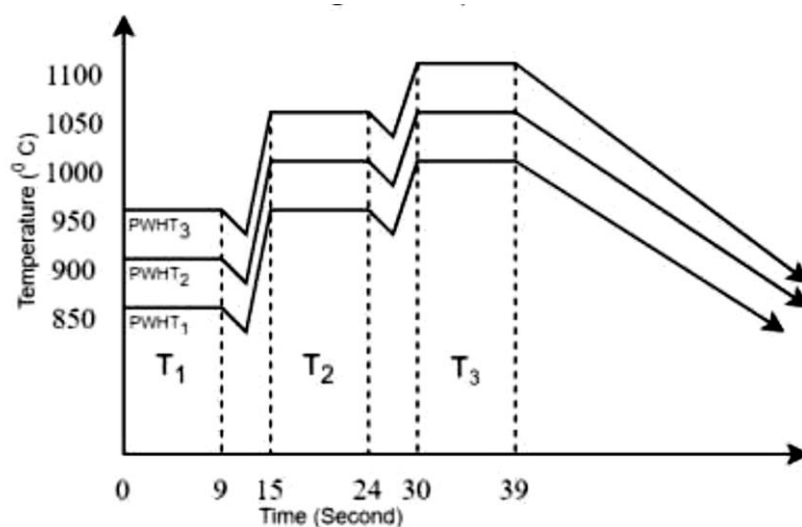
Figure 6. PWHT Temperature Diagram
