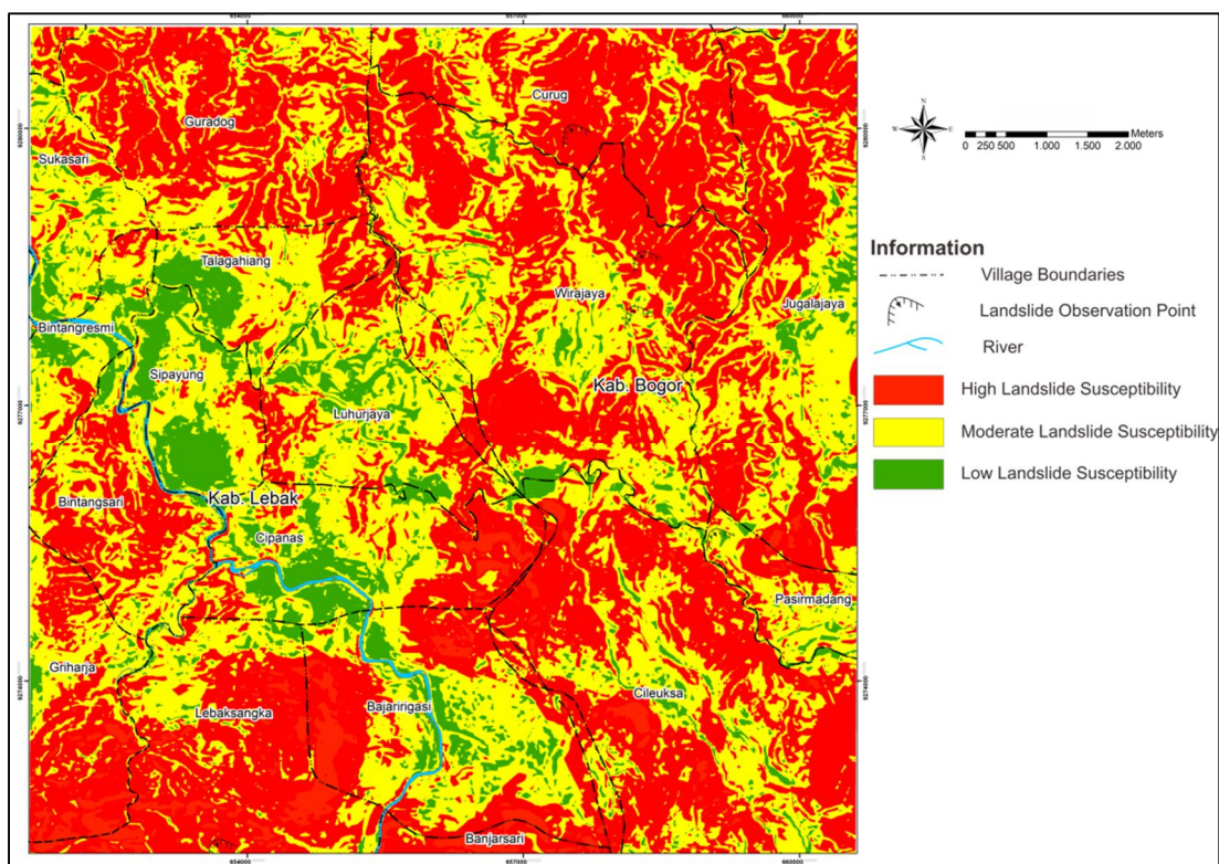
Figure 9. Landslide susceptibility map
