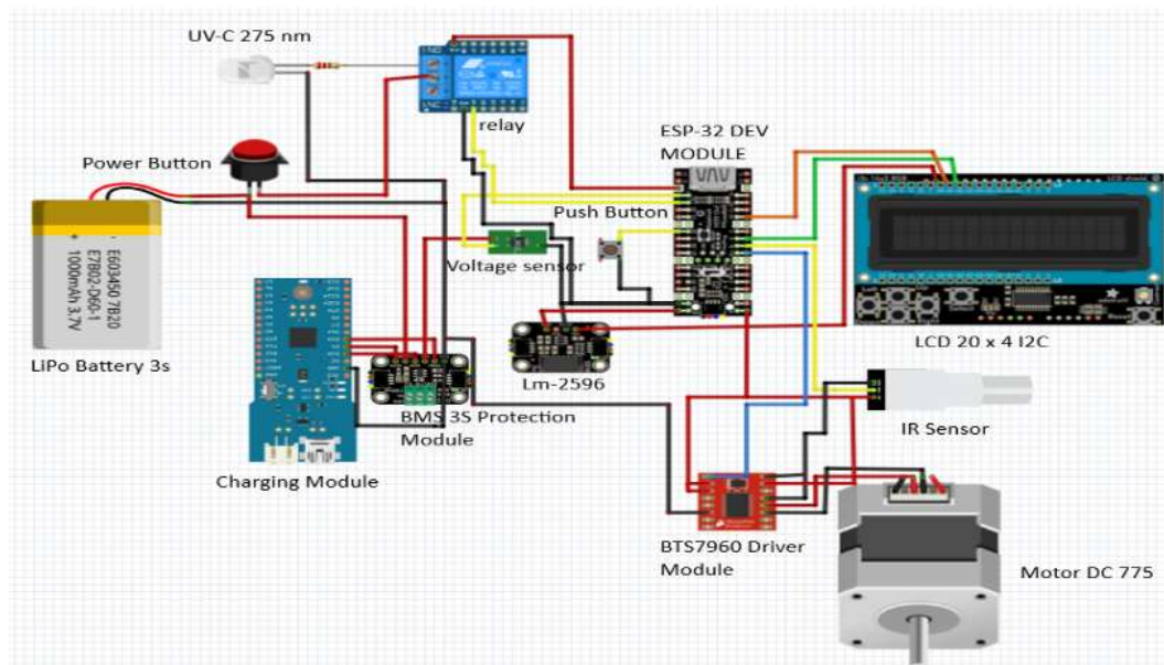
Figure 2. Wiring diagram of the NECIS system.
