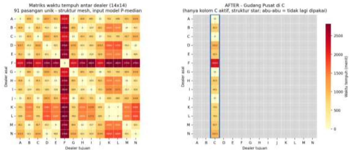
Figure 1. Travel-time matrix before and after selecting Dealer C as the single Depot.
