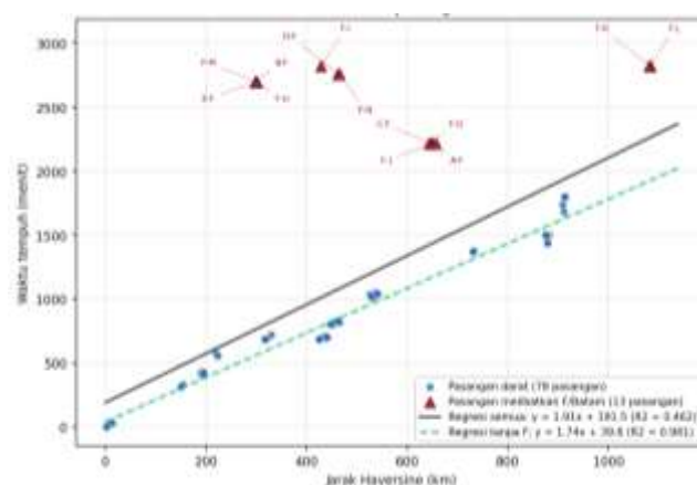
Figure 4. Relationship between Haversine distance and inter-dealer travel time.
