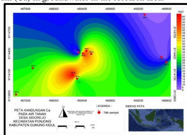
Figure 8. Groundwater Quality Distribution Map Based on Ca Content
