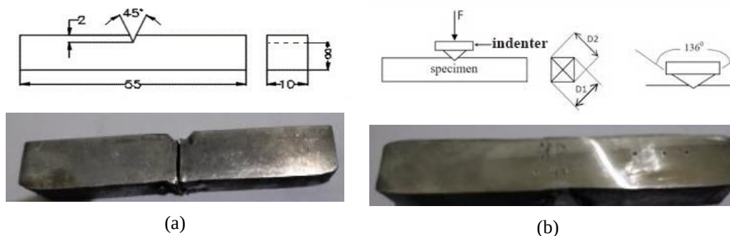
Figure 2. a) Impact test specimen, b) hardness test specimen.
