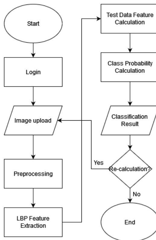
Figure 2. System Flowchart
