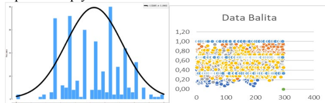
Gambar 7. Distribusi Data
