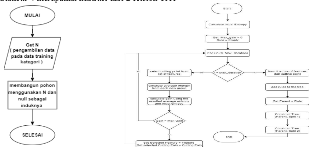
Gambar 4. Decision Tree
