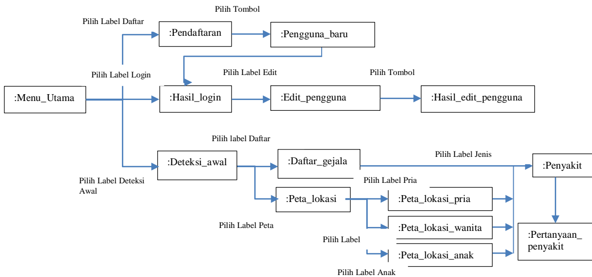
Gambar 7. Interface flow diagram
