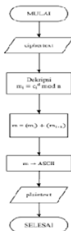
Gambar 3. Flowchart Dekripsi Algoritma RSA
