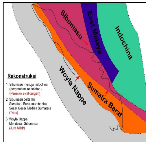
Figure 2. The constituent continental block of Sumatera Island (Modification from [6])
